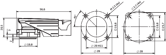
Mounting hole
