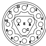
mating view
