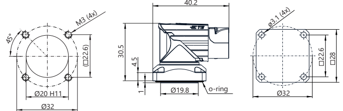
Mounting hole
