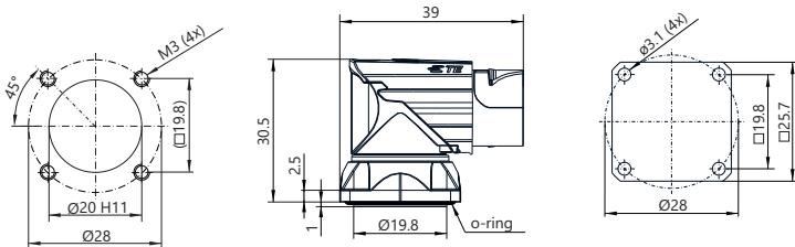
Mounting hole
