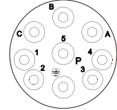
mating view
