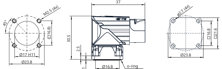
Mounting hole
