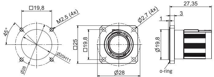
Mounting hole
