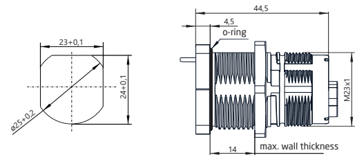
Mounting hole
